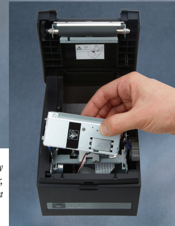
The CT-S310II features easy maintenance for Cutter, Print Head and Platen
